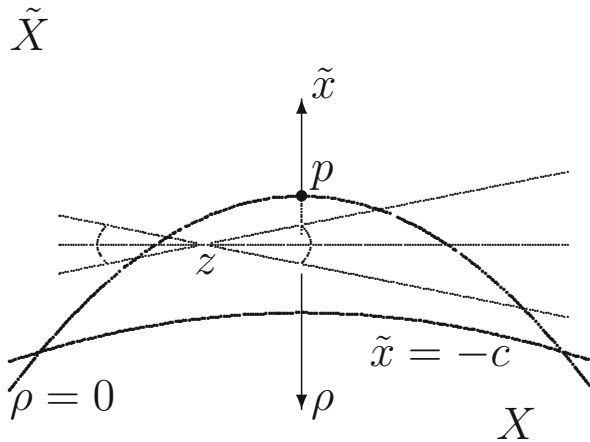
Fig. 1 The functions \rho and \tilde{x} when the background is flat space \tilde{X} . The intersection of \rho \geq 0 and x_c > 0 (where x_c = \tilde{x} + c , so this is the region \tilde{x} > -c ) is the lens shaped region O_p . Note that, as viewed from the superlevel sets, thus from O_p , \tilde{x} has concave level sets. At the point z , L integrates over geodesics in the indicated small angle. As z moves to the artificial boundary x_c = 0 , the angle of this cone shrinks like Cx_c so that in the limit the geodesics taken into account become tangent to x_c = 0
