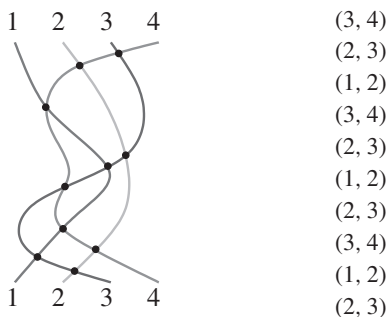
Figure 6. Illustration of the proof of Theorem 4.1.
