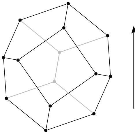
Figure 11. The 3-dimensional associahedron.
