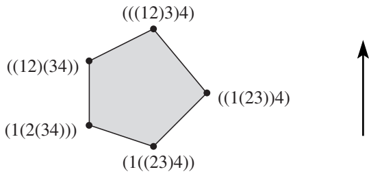
Figure 10. The two dimensional associahedron.
