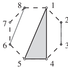
Figure 4. A noncrossing partition of the set [8] .
