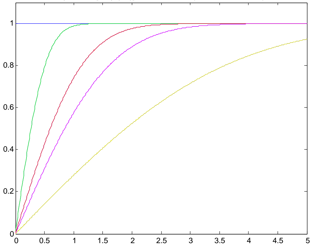
A plot of \text{Erf}[x/\sqrt{4kt}] at various times ( t=0, t=.1, t=.5, t=1, t=5 )
