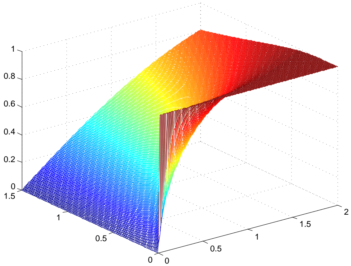
A plot of \text{Erf}[x/\sqrt{4kt}] , a solution of the heat equation on the half line
