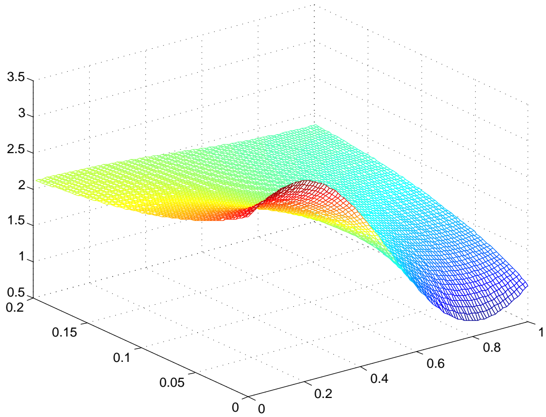
Another solution of the heat equation on 0 < x < l , Neumann BC
