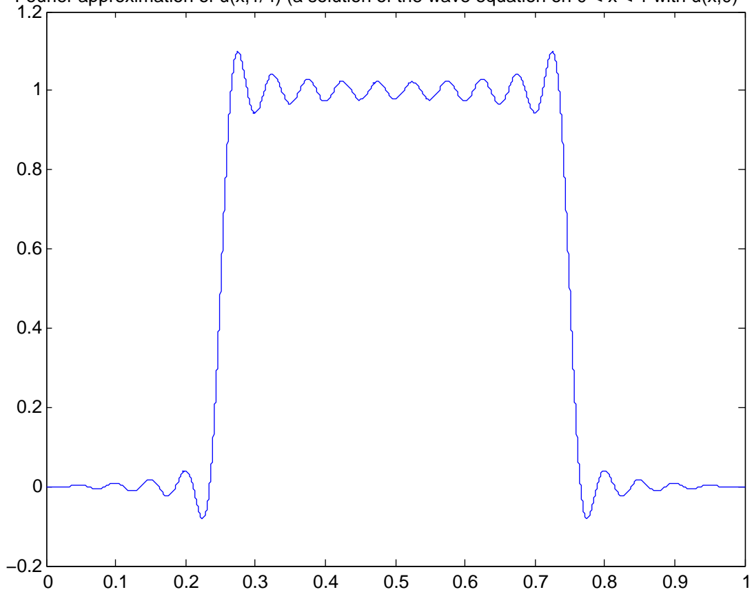
Fourier approximation of u(x, 1/4) (a solution of the wave equation on 0 < x < 1 with u(x, 0) = 1 )
