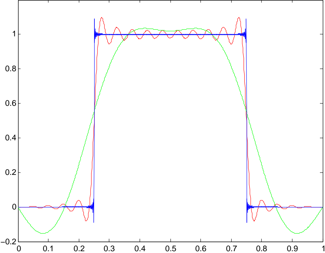
Approximation (3, 20, 500 terms) of the Fourier series solving (WE) on 0 < x < 1 with IC u(x,0)=1 : T = .25
