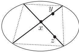
FIGURE 1. Comparing to a quadrilateral
