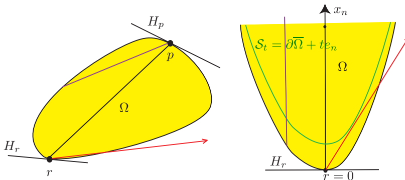
FIGURE 5. Horospheres.
