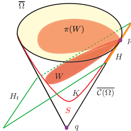
FIGURE 8. Hilbert hypersurface
