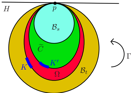
FIGURE 10. Comparing \Omega to \mathcal{B}_t and \mathcal{B}_s .
