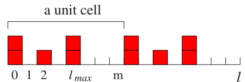
FIG. 4. (Color online) The graphic representation of an occupation distribution (n_0, \dots, n_{10}) = (2, 0, 1, 0, 2, 0, 0, 0) for the \Phi_{5/8; \mathbb{Z}_5^{(2)}} state with n=5 and m=8 . l_{\max}=4 for such a distribution.
