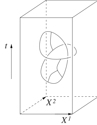
FIG. 9. A general quasiparticle tunneling process.
