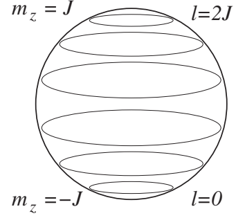
FIG. 2. The 2J+1 orbital on a sphere forms an angular-momentum J representation of the O(3) rotation.
