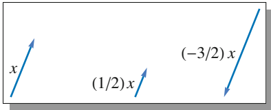
Scalar multiplication.
