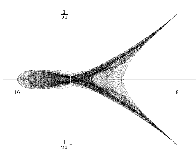
Figure 8: The plottings of the set (9) for some family of knots [Oku02]
