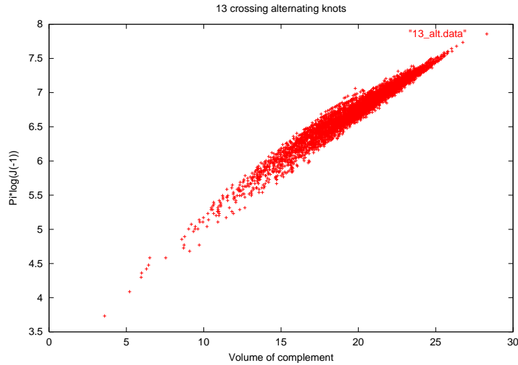
Figure 4: The distribution of pairs of the hyperbolic volume of knot complements and \pi \log V_K(-1) for alternating knots with 13 crossings [Dun.www].
