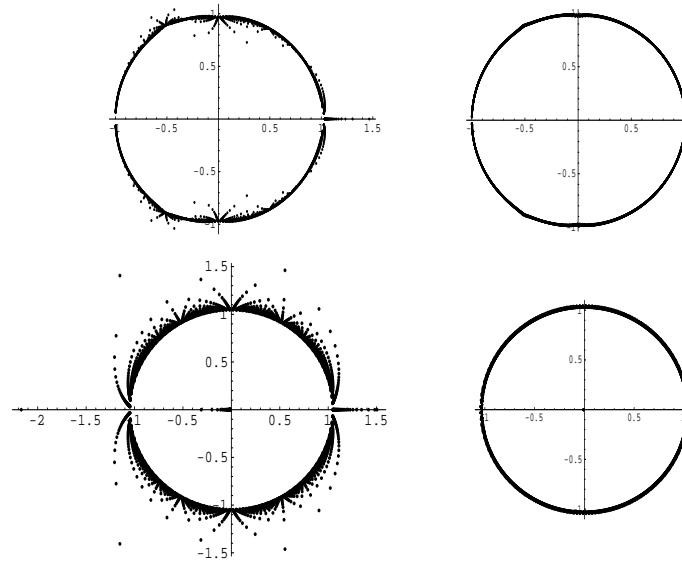
Figure 3: The upper pictures show the distribution of zeros of the Jones polynomial for n -twist knots, with n from 1 to 50 and from 51 to 100, respectively [Lin.www]. The lower pictures show the distribution of zeros of the Jones polynomial for (2, 2n - 1) torus knots, with n from 1 to 50 and from 51 to 100, respectively [Lin.www]. See [Lin.www] for further pictures for (3, 3n + 1) and (3, 3n + 2) torus knots.
