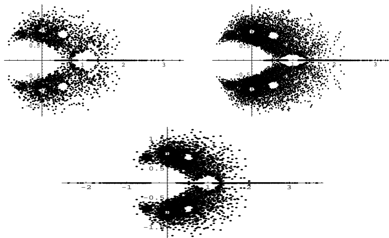
Figure 2: The upper pictures show the distribution of zeros of the Jones polynomial for alternating knots of 11 and 12 crossings [Lin.ww]. The lower picture shows the distribution of zeros of the Jones polynomial for 12 crossing non-alternating knots [Lin.ww]. See [Lin.ww] for further pictures for alternating knots with 10 and 13 crossings.
