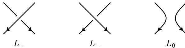
Figure 1: Three links L_+, L_-, L_0
