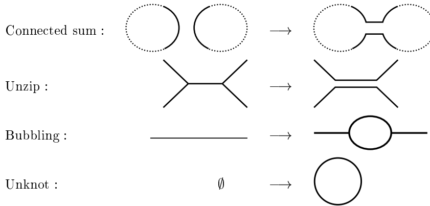
Figure 21: Four operations of KTG's [BaTh01b]. The left hand side of the connected sum denotes a disjoint union of two separate graphs.
