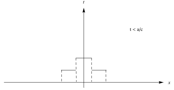
Figure 4: The solution for 0 < t < a/c .
