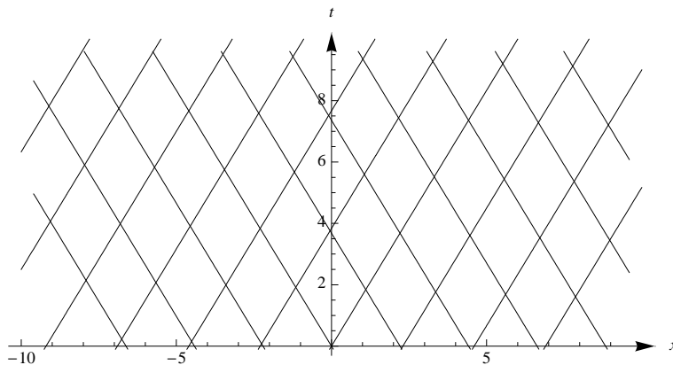
Figure 1: Characteristic lines for the wave equation with c = 0.6 .
