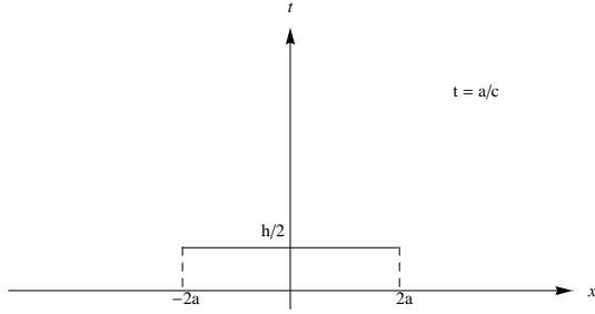
Figure 5: The solution at t = a/c .
