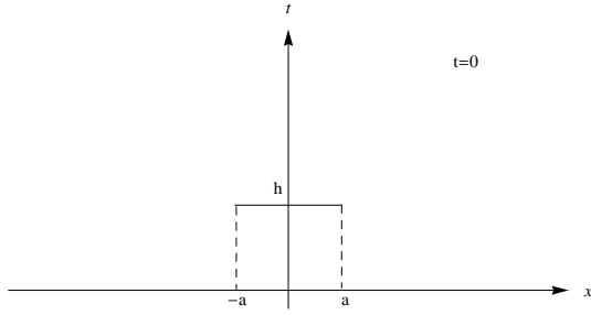
Figure 3: The solution at t = 0 .
