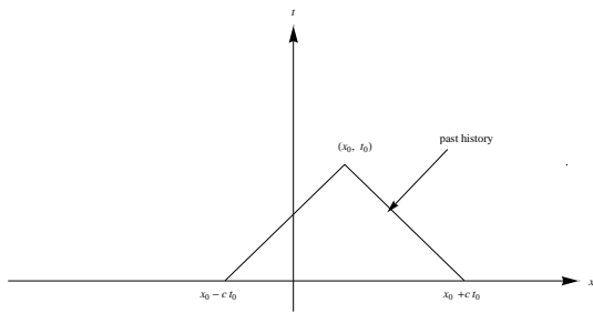
Figure 7: Domain of dependence for (x_0, t_0) .
