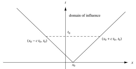
Figure 8: Domain of influence of x_0 .
