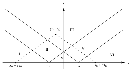
Figure 9: Regions where u has different values.
