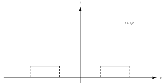
Figure 6: The solution for t > a/c .
