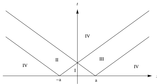
Figure 2: Regions where u has different values.
