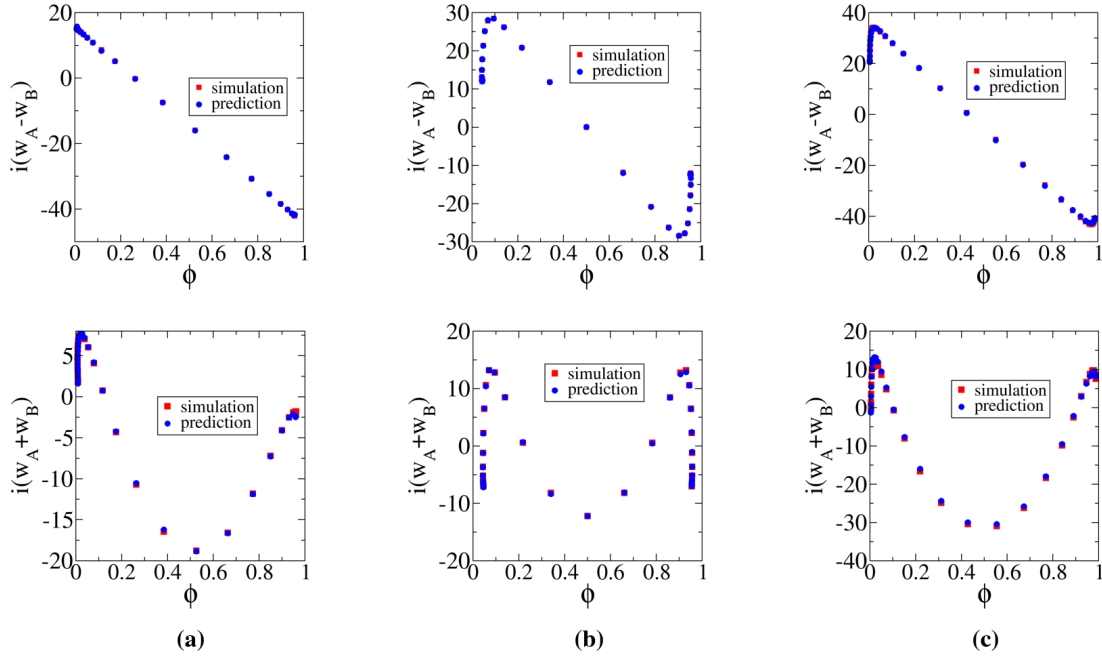
FIG. 7. Partial saddle points of w_A^*[\phi] - w_B^*[\phi] (top row) and w_A^*[\phi] + w_B^*[\phi] (bottom row) predicted by ML model (blue) and from DE-AF field theory simulation (red) for different density profiles. (a) A saddle-point density profile at \chi N = 30 , f = 0.26 , and L = 5.0R_g . (b) A non-saddle point density profile at \chi N = 34.6859 , f = 0.50 , and L = 4.9836R_g . (c) A non-saddle point density profile at \chi N = 38.6934 , f = 0.42 , and L = 2.9074R_g .
