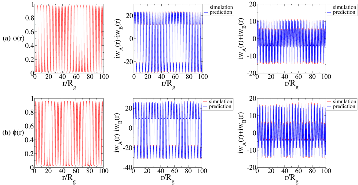
FIG. 9. Non-saddle point density profiles \phi(\mathbf{r}) (left column) at a high spatial resolution of 2048 and the corresponding partial saddle points iw_A^*(\mathbf{r}) (middle column) and iw_B^*(\mathbf{r}) (right column) predicted by the ML model (blue) and from simulations (red) for two conditions: (a) \chi N = 30 , f = 0.40 , and 205.19R_g . (b) \chi N = 34 , f = 0.37 , and 210.82R_g . Here we only show a portion of the boxes for better visual clarity.
