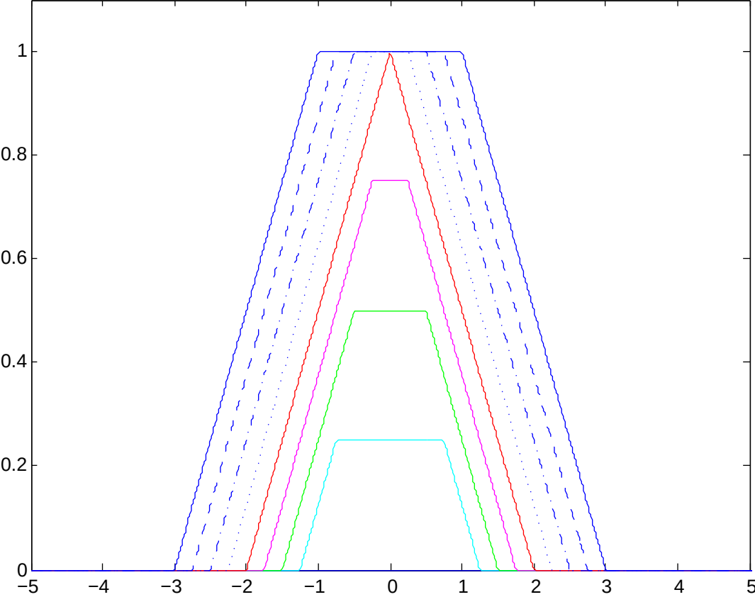
Plots of the hammer blow ( c=a=1 ) at t=0,.25,.5,.75,1,1.25,1.5,1.75,2
