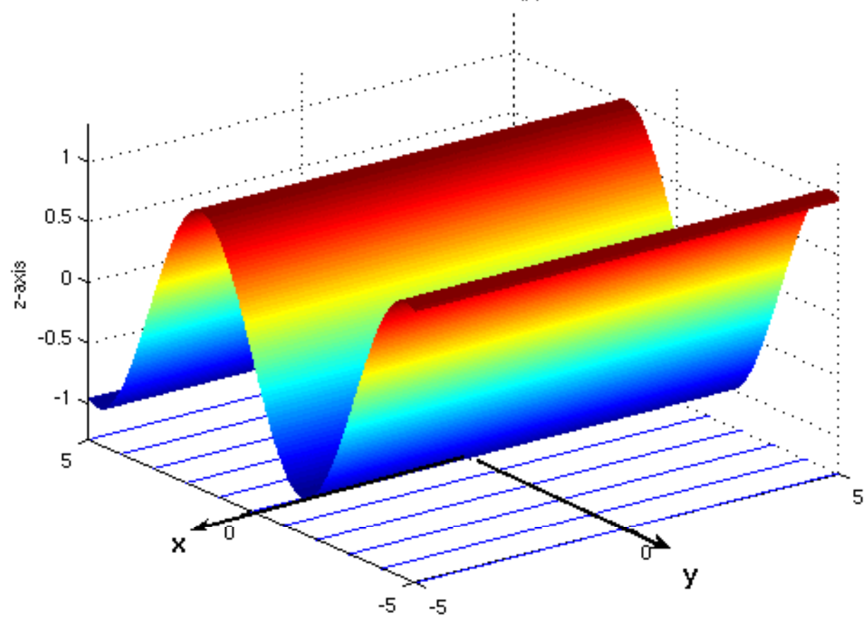
The surface z=\sin(y)
