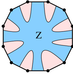
FIGURE 1. A windmill configuration in a 2-cell.
