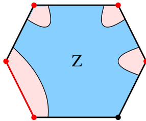
FIGURE 2. A windmill created by \partial A .
