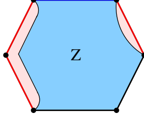
FIGURE 3. A windmill created by \partial A .
