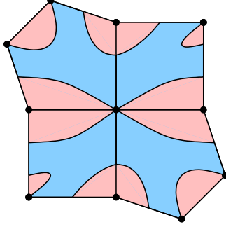
FIGURE 4. An example of branching in \Gamma'
