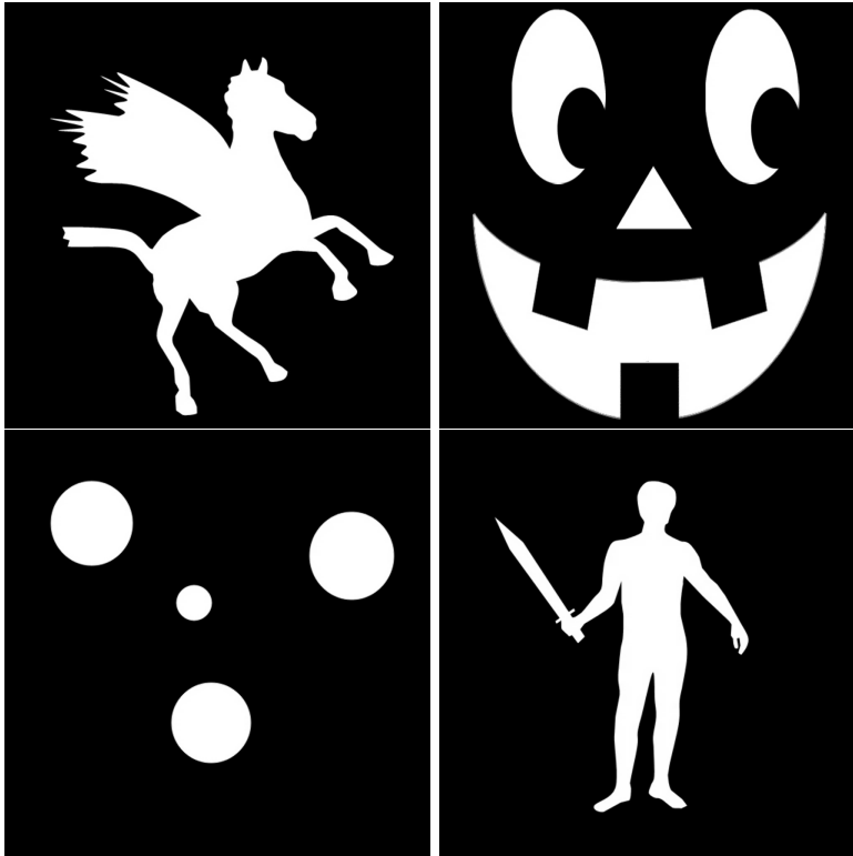
FIGURE 1. Several image examples used to construct interpolations.
