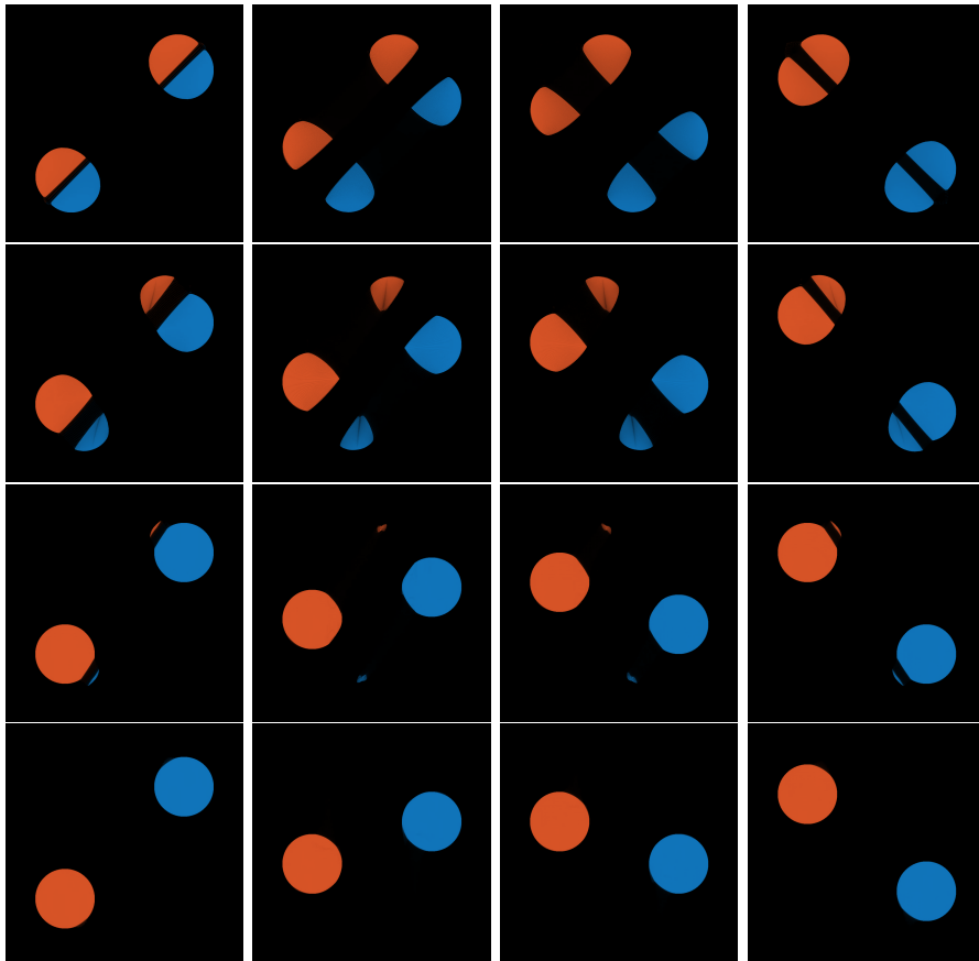
FIGURE 4. Optimal transport with different cost functions. Each row depicts the optimal trajectory for a cost of the form (14). Row 1: p_1 = 2 , p_2 = 2 ; Row 2: p_1 = 1.75 , p_2 = 2.25 ; Row 3: p_1 = 1.5 , p_2 = 2.5 ; Row 4: p_1 = 1.1 , p_2 = 3 . Colors represent an assignment: orange pixels move to the upper left disk while blue pixels move to the lower right disk.
