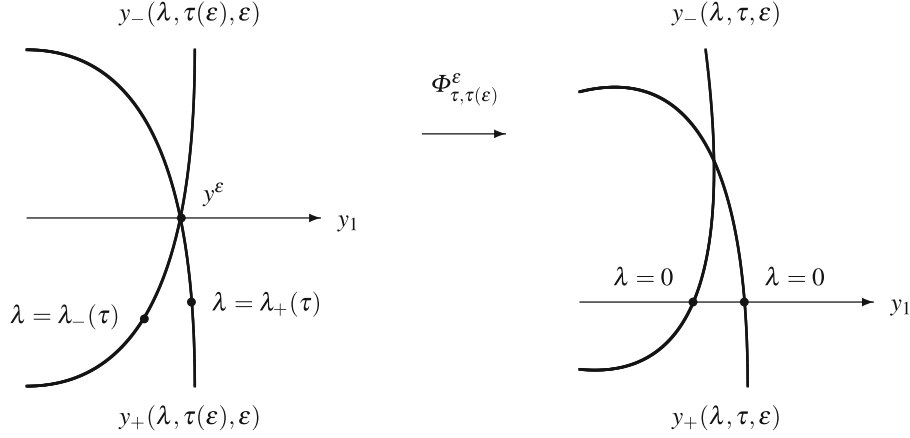
Fig. 10.2 Slices of the invariant manifolds at time \tau(\epsilon) and their images under the flow \Phi_{\tau, \tau(\epsilon)}^\epsilon for a time \tau \sim \tau(\epsilon)
