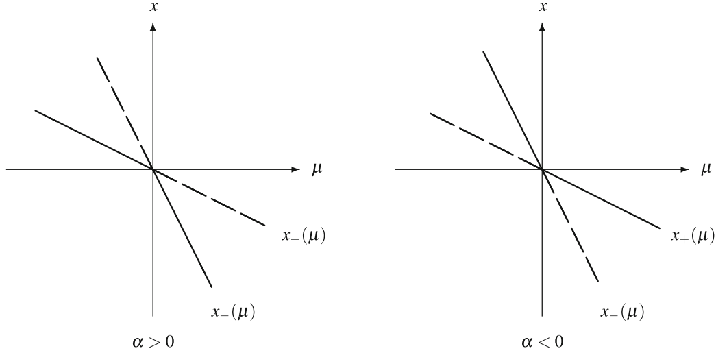
Fig. 9.3 Transcritical bifurcation diagrams
